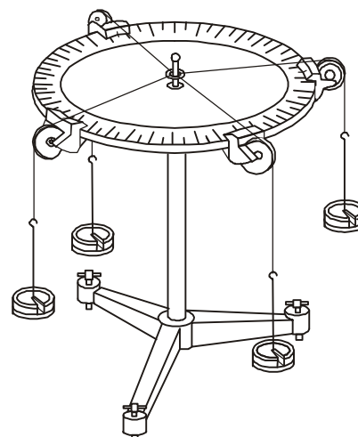
Figure 1.2 – Force table.
